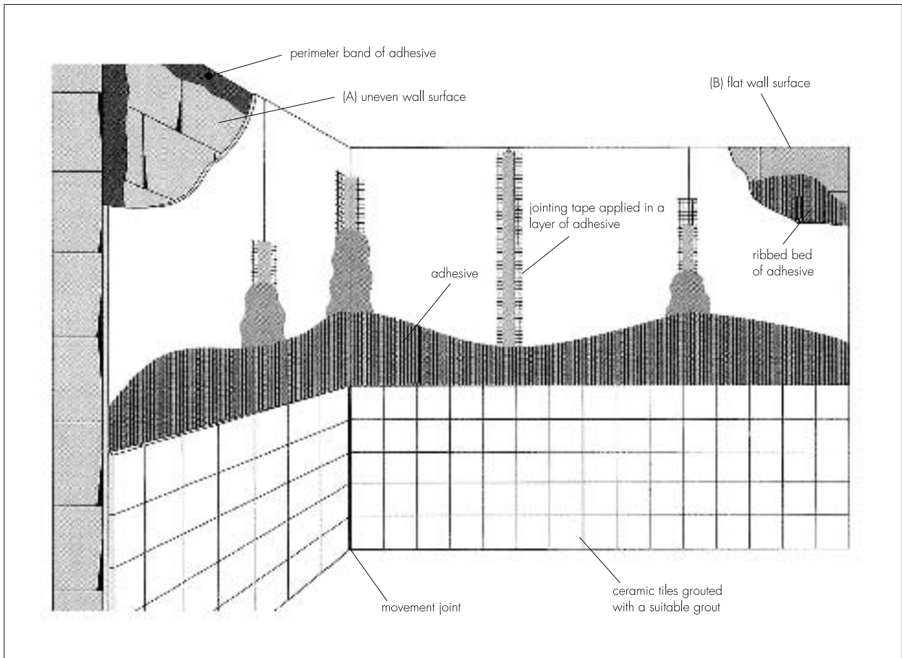
Figure 1 Installation — direct bonding
