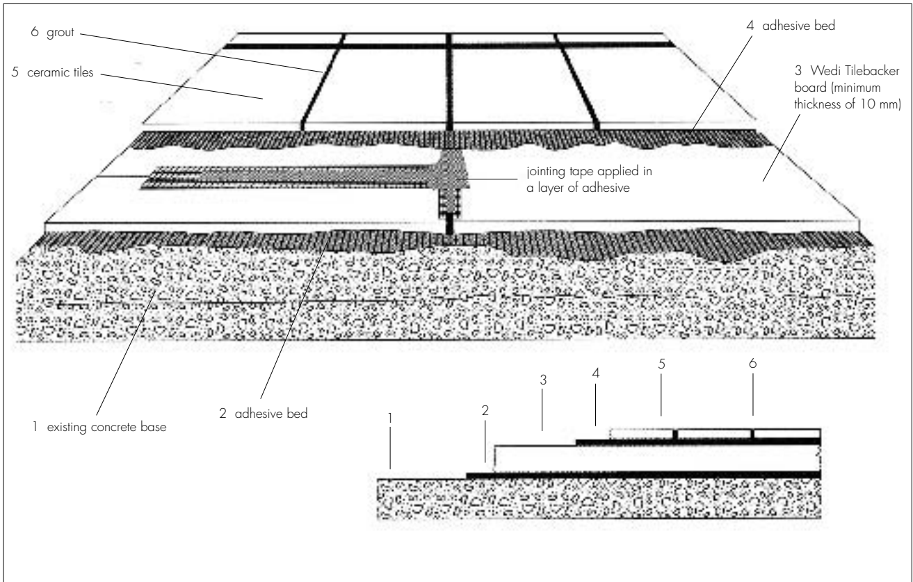
Figure 3 Installation — concrete floors
